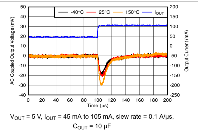
Figure 6-18. Load Transient, 45-mA to 105-mA Rising Edge
