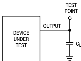
Figure 2. Test Circuit
