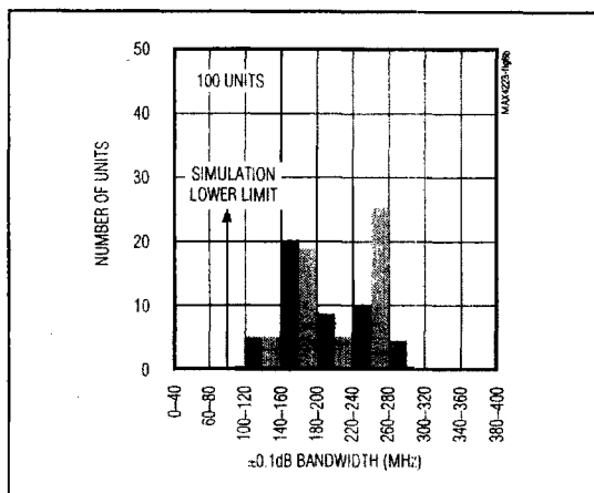
Figure 6b. MAX4224 ±0.1dB Bandwidth Distribution
