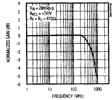
MAX4227/MAX4228 SMALL-SIGNAL GAIN vs. FREQUENCY ( A_{VCL} = +2 )
