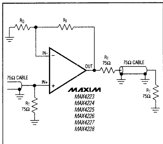
Figure 3. Video Line Driver
