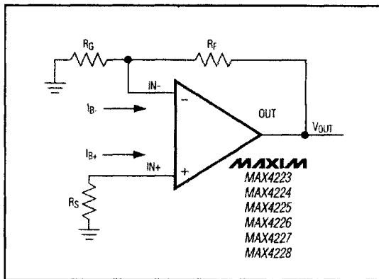
Figure 2. Output Offset Voltage
