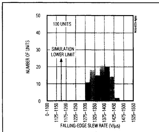
Figure 6d. MAX4224 Falling-Edge Slew-Rate Distribution
