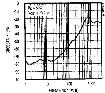
MAX4227/MAX4228 CROSSTALK vs. FREQUENCY
