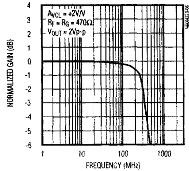
MAX4227/MAX4228 SMALL-SIGNAL GAIN vs. FREQUENCY ( A_{VCL} = +2 )
