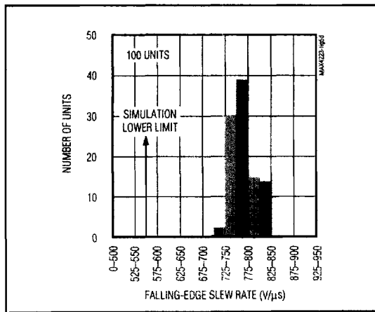
Figure 5d. MAX4223 Falling-Edge Slew-Rate Distribution
