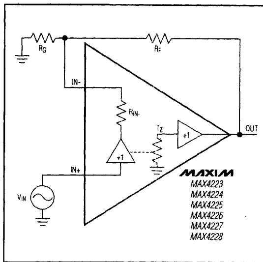
Figure 1. Current-Feedback Amplifier
