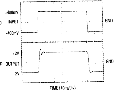
MAX4224/MAX4227/MAX4228 LARGE-SIGNAL PULSE RESPONSE ( A_{vCL} = +5 )
