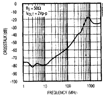
MAX4225/MAX4226 CROSSTALK vs. FREQUENCY
