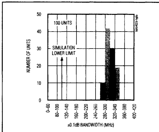
Figure 5b. MAX4223 ±0.1dB Bandwidth Distribution
