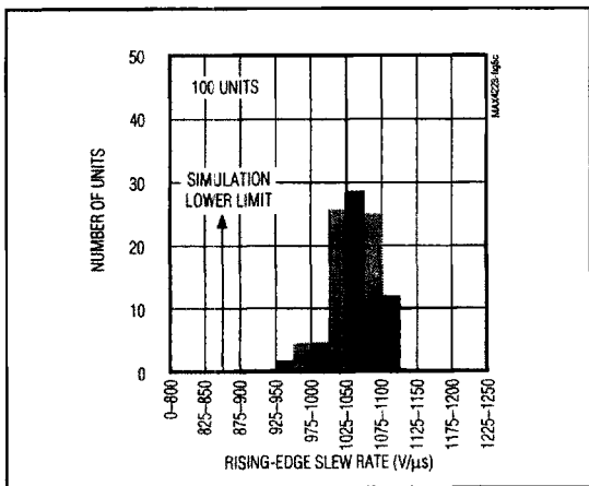
Figure 5c. MAX4223 Rising-Edge Slew-Rate Distribution
