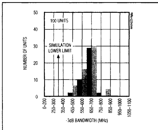
Figure 6a. MAX4224 -3dB Bandwidth Distribution
