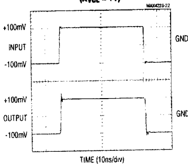
MAX4223/MAX4225/MAX4226 SMALL-SIGNAL PULSE RESPONSE ( A_{vCL} = +1 )
