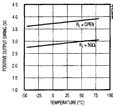
POSITIVE OUTPUT SWING vs. TEMPERATURE
