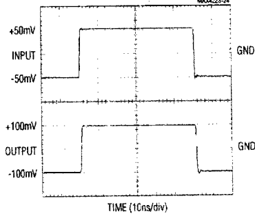
MAX4224/MAX4227/MAX4228 SMALL-SIGNAL PULSE RESPONSE ( A_{vCL} = +2 )
