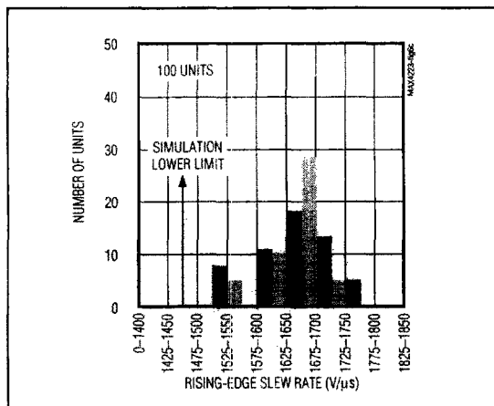
Figure 6c. MAX4224 Rising-Edge Slew-Rate Distribution
