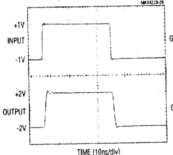
MAX4224/MAX4227/MAX4228 LARGE-SIGNAL PULSE RESPONSE ( A_{vCL} = +2 , C_L = 10pF )
