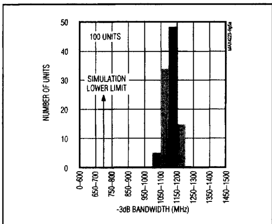
Figure 5a. MAX4223 -3dB Bandwidth Distribution
