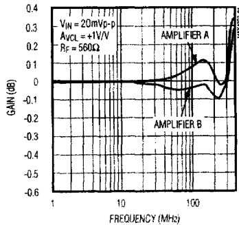
MAX4225/MAX4226 GAIN MATCHING vs. FREQUENCY ( A_{VCL} = +1 )
