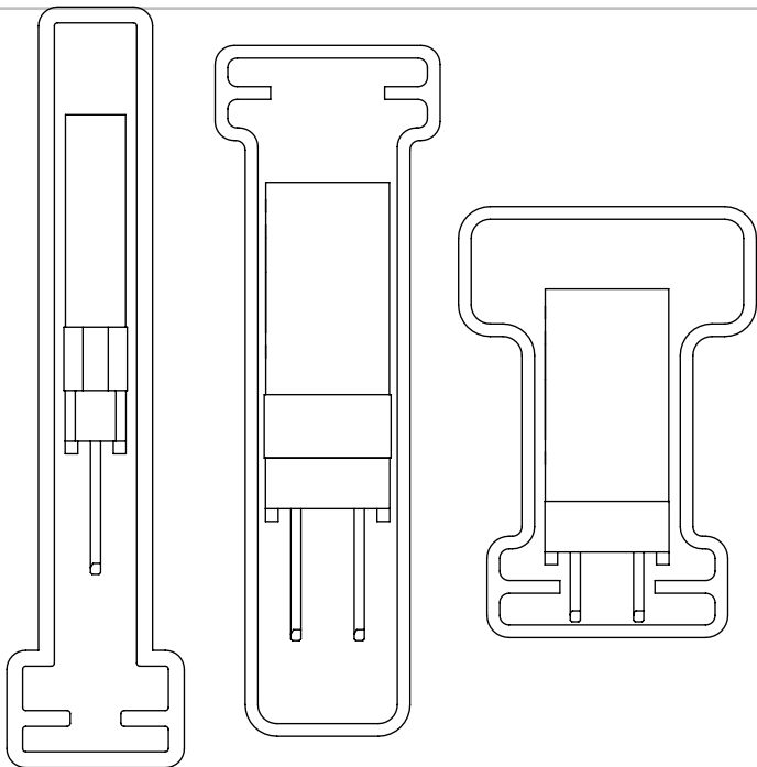
FIG 7 TUBE VIEWS
