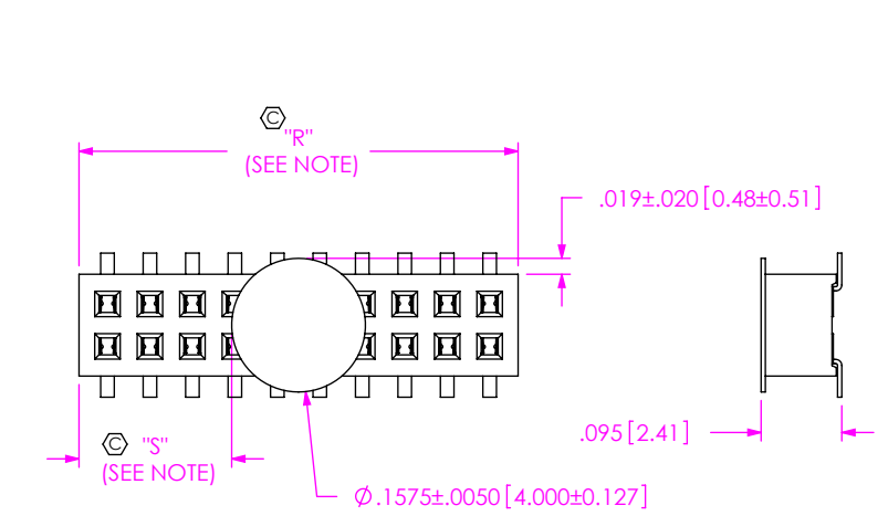
FIG 5 -K: POLYIMIDE FILM PAD (AVAILABLE ON POSITION 05 THRU 50 ONLY) (NOT AVAILABLE WITH -P OR -PA OPTIONS)
