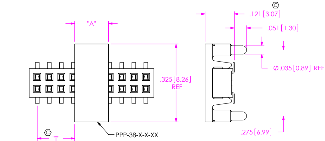
FIG 4 -PA: PICK & PLACE PAD WITH ALIGNMENT PINS (NOT AVAILABLE WITH -P, -A OR -K OPTIONS)
