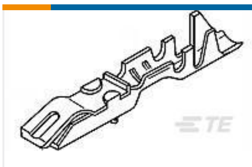
TE Part #87165-1 LOCKING CLIP ASSY .025 SQ LP
