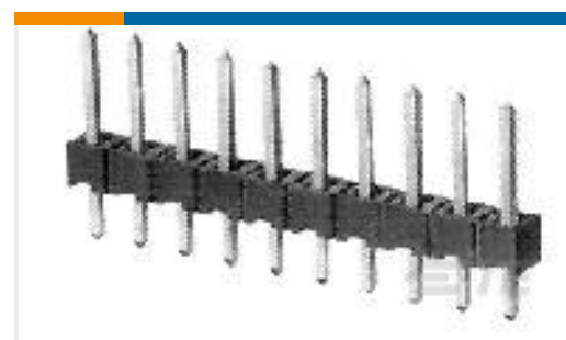
TE Part #825433-7 MOD 2 PINHDR 1X7 P.
