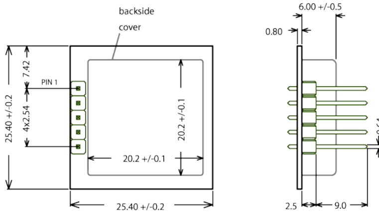
Fig. 3: Mechanical data
