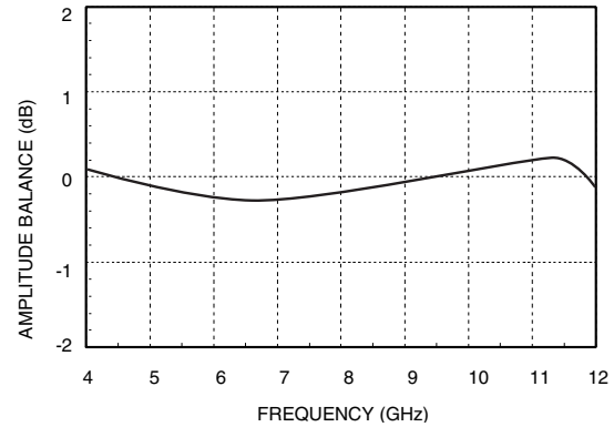
Amplitude Balance
