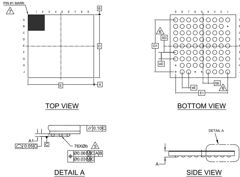
Figure 1276-Ball WLCSP Package Outline
