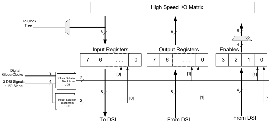
Figure 6. Port Interface
