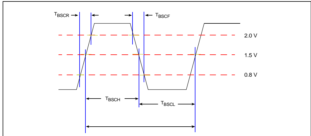
Figure 35. T_{BSIS1} and T_{BSIH1} Input Setup and Hold Waveforms
