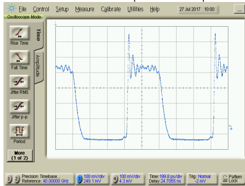
NLTL Output for 1GHz +25 dBm Square Wave Input
