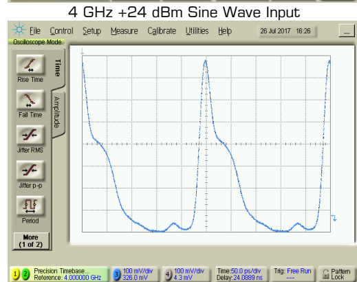
NLTL Output for 4GHz +24 dBm Sine Wave Input
