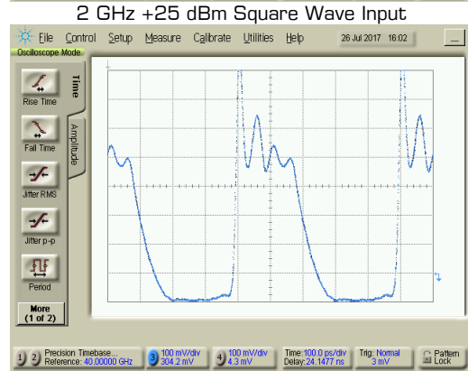
NLTL Output for 2GHz +25 dBm Square Wave Input
