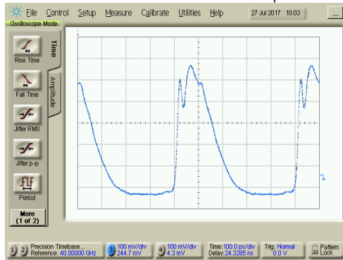
NLTL Output for 2GHz +25 dBm Sine Wave Input
