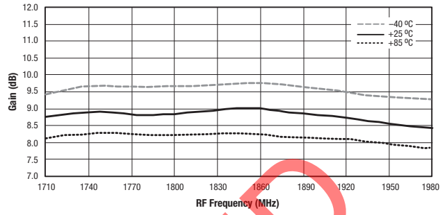
Figure 4. Mixer Gain vs Frequency and Temperature
