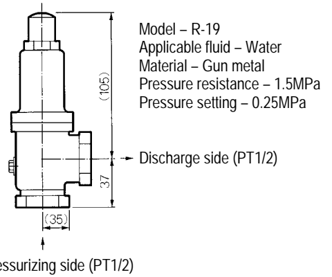
Figure 13 External Dimensions of Safety Valve (Unit: mm)
