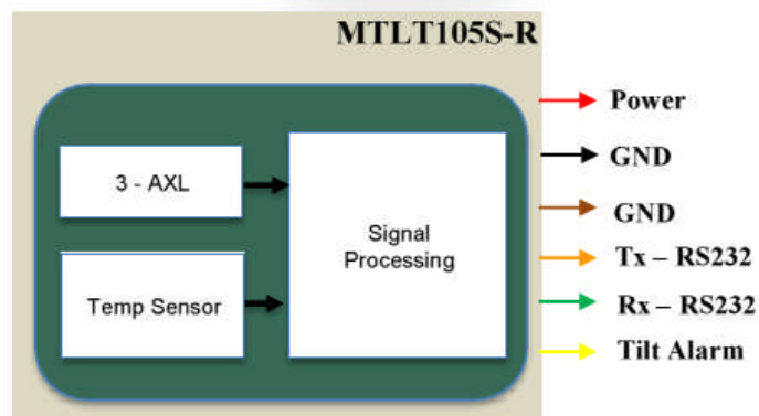
Platform Leveling
