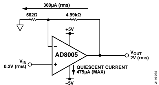
Figure 35. Saving Power by Increasing Feedback Resistor Network
