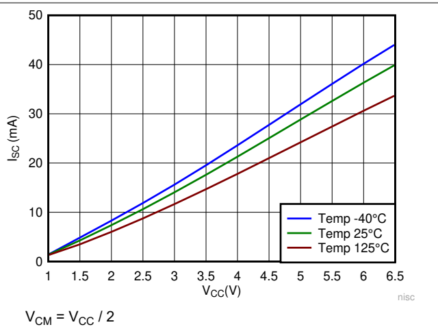
图 6-24. Output Short Circuit (Sink) vs V_{CC}
