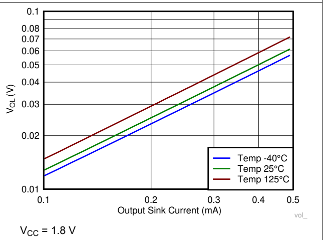
图 6-20. Output Voltage Low vs Output Sink Current
