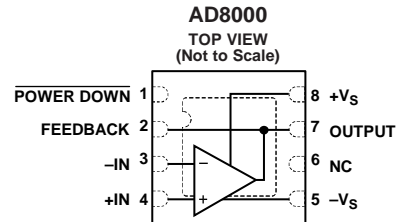
Figure 1. 8-Lead AD8000 , 3 mm \times 3 mm LFCSP (CP-8-13)
