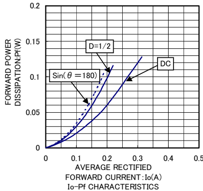
Io-Pf CHARACTERISTICS
