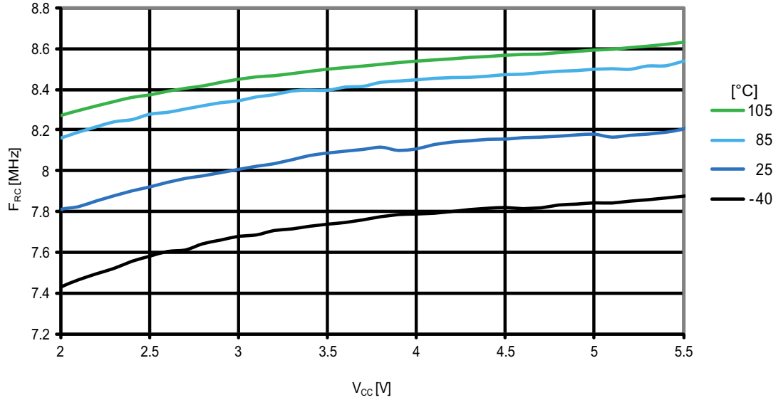
Figure 31-153. ATmega1284P: Calibrated 8MHz RC oscillator vs. V_{CC}
