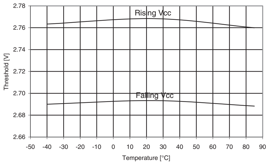
Figure 30-81. ATmega164PA: BOD threshold vs. temperature ( V_{BOT} = 2.7V )
