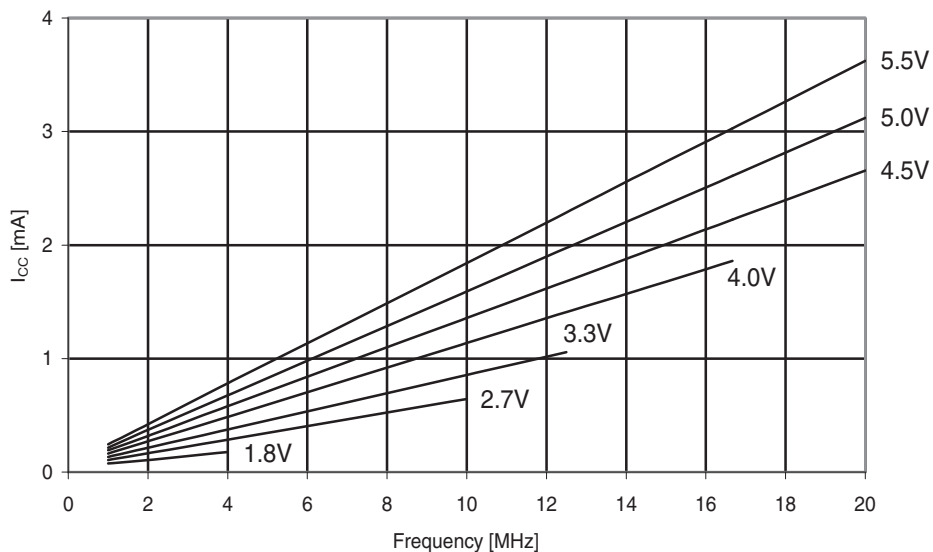
Figure 30-154. ATmega324PA: Idle supply current vs. V_{CC} (1 - 20MHz)
