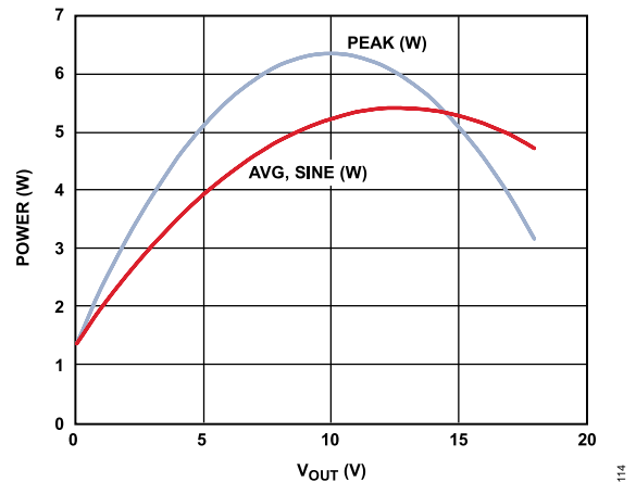
Figure 73. Average Sine and Peak Power vs. V_{OUT} , V_S = \pm 20 V, R_L = 20 \Omega
