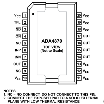
Figure 3. Pin Configuration
