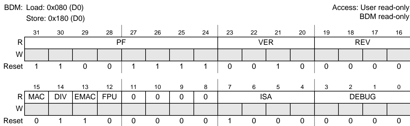
Figure 2-18. D0 Hardware Configuration Info
