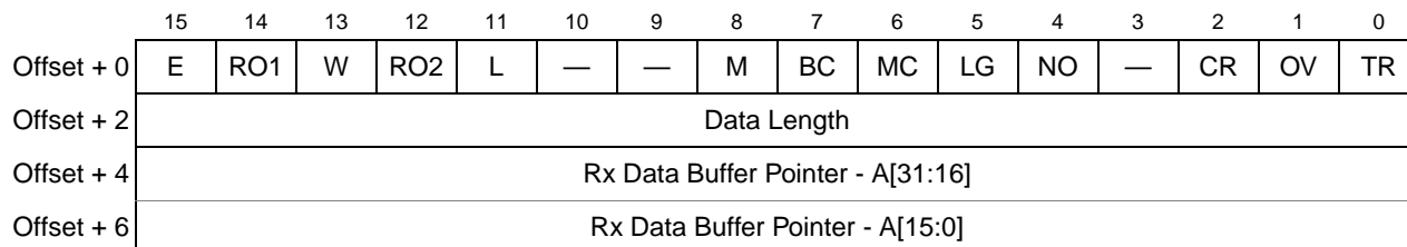
Figure 17-25. Receive Buffer Descriptor (RxB)
