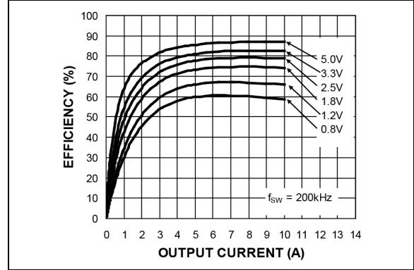
FIGURE 2-30: Efficiency ( V_{IN} = 75V ) vs. Output Current (MIC2104).
