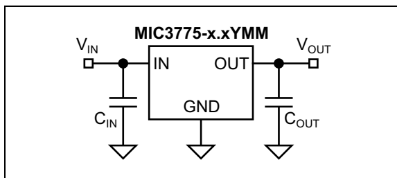
FIGURE 4-1: Capacitor Requirements.
