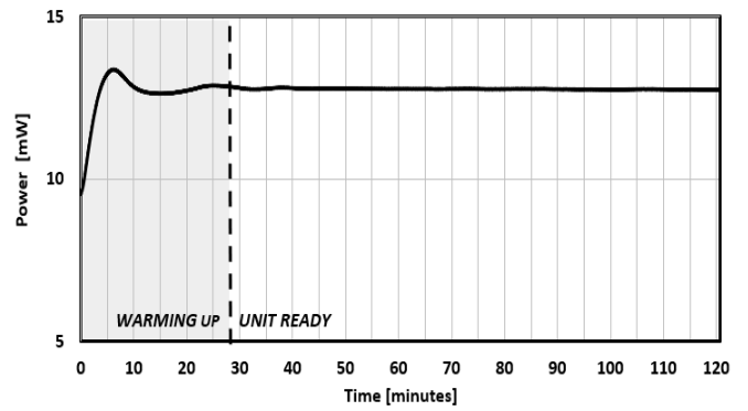
FIG. 4: WARM-UP TIME
