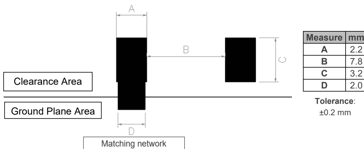
Footprint dimensions for the single booster.
