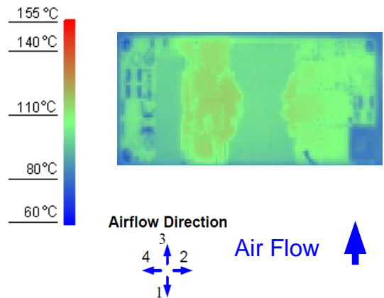
Figure 12. Thermal Image for Airflow Direction 3 (48A output, 85°C ambient, 400 LFM, typical Vin, open frame unit)
