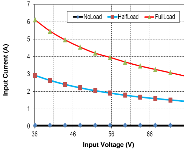
Figure 3. Input Characteristics (25°C)
