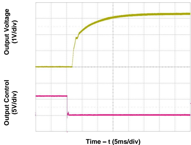
Figure 6. Start-Up from Enable Control (typical Vin, zero load, 1,000µF external output capacitance)
