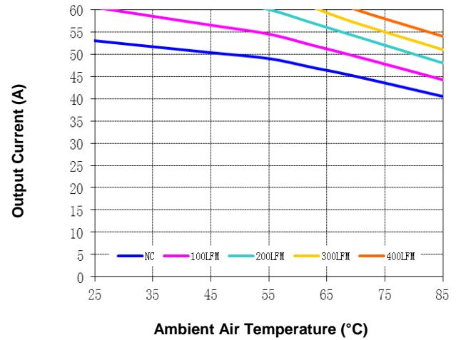
Figure 10. Current Derating Curve for Airflow Direction 3 (Ref. Fig. 12 for Airflow Direction; typical Vin, baseplate, solder interface)
