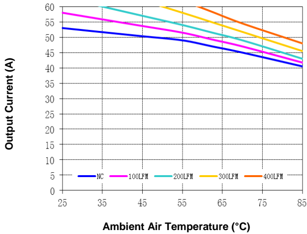
Figure 9. Current Derating Curve for Airflow Direction 3 (Ref. Fig. 12 for Airflow Direction; typical Vin, open frame, solder interface)
