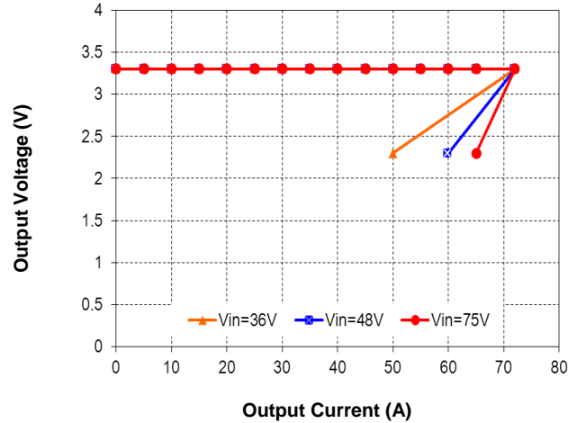
Figure 4. Output Characteristics (25°C)
