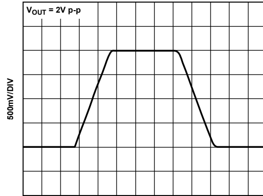
Figure 32. Large Signal Pulse Response, V_S = \pm 2.5 V
