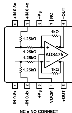
Figure 2. 10-Lead MSOP
