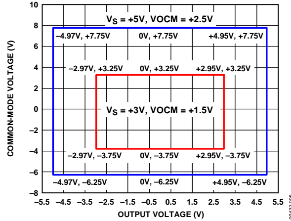
Figure 8. Input Common-Mode Voltage vs. Output Voltage, V S = +5 V and +3 V
