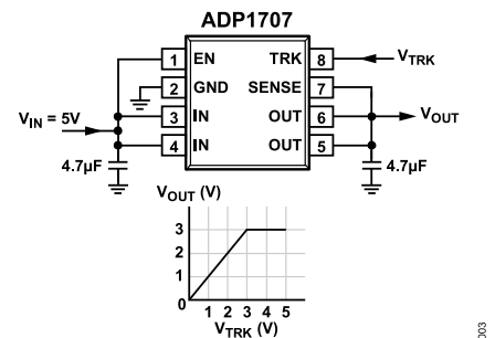
Figure 2. ADP1707 with Output Voltage Tracking
