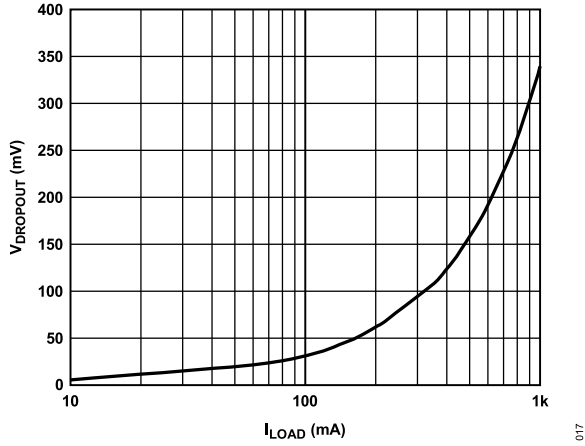
Figure 16. Dropout Voltage ( V_{DROPOUT} ) vs. Load Current ( I_{LOAD} )
