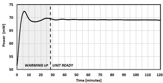
FIG. 9: WARM-UP TIME
