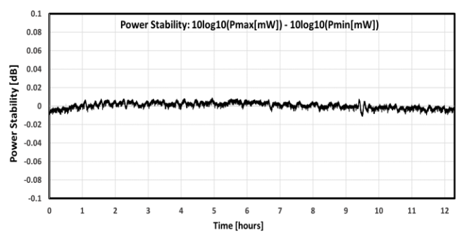
FIG. 8: ISB2 TYPICAL POWER STABILITY
