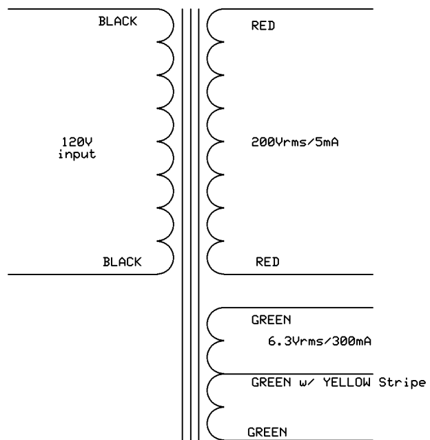
Primary and Secondary Schematic
