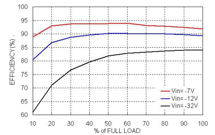
ASR01-12S05 Efficiency VS Output Load
