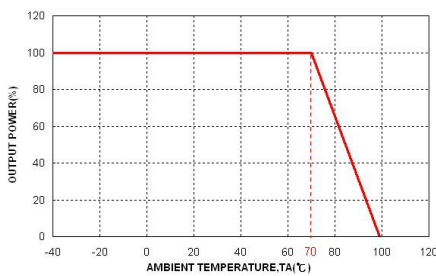
ASR01-12S05 Derating Curve
