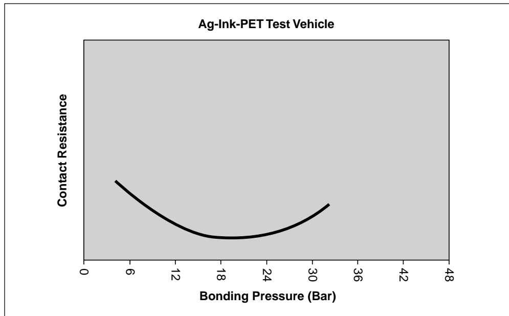
Figure 1. Graph of relative contact resistance vs. bonding pressure using polyester flexible printed circuitry with silver ink circuit lines bonded to printed circuit board with gold/nickel/copper circuit lines.
