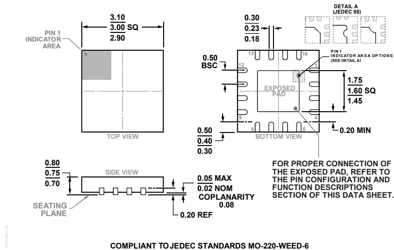
COMPLIANT TO JEDEC STANDARDS MO-220-WEED-6 Figure 117. 16-Lead Lead Frame Chip Scale Package [LFCSP] 3 mm × 3 mm Body and 0.75 mm Package Height (CP-16-22) Dimensions shown in millimeters
