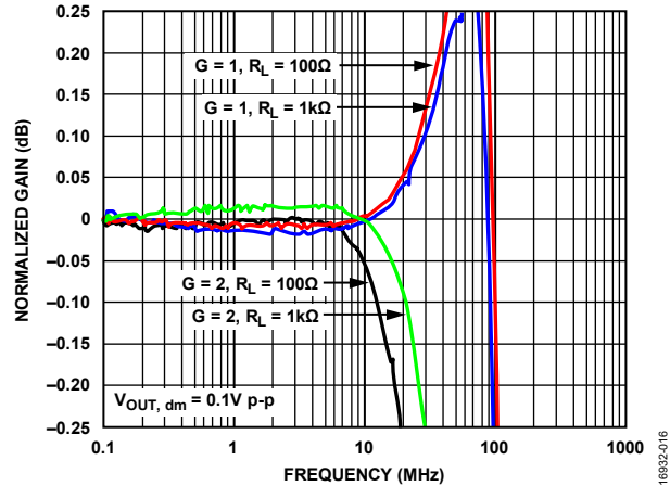
Figure 13. 0.1 dB Flatness Small Signal Frequency Response for Various Gains and Loads
