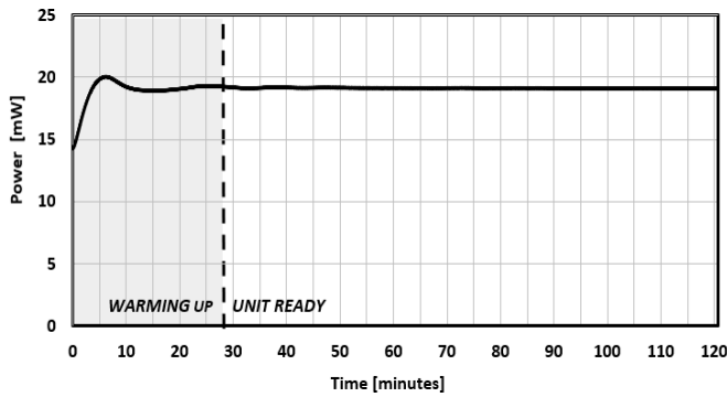
FIG. 9: WARM-UP TIME
