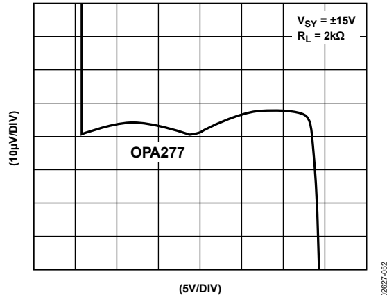
Figure 52. Gain Linearity
