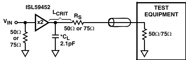
FIGURE 32D. BACKLOADED TEST CIRCUIT FOR 150Ω VIDEO CABLE APPLICATION
