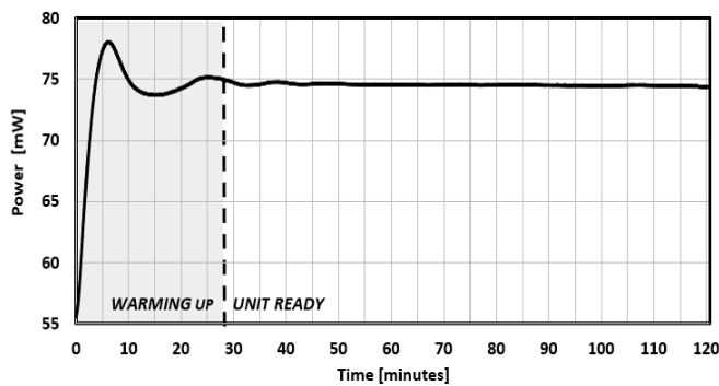
FIG. 9: WARM-UP TIME
