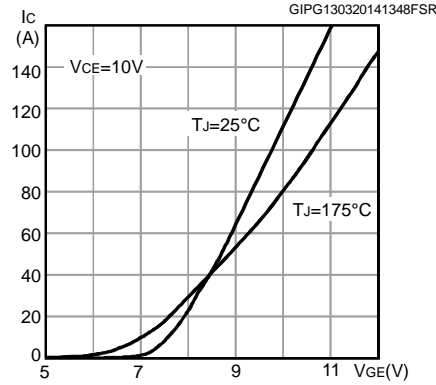
Figure 10: Transfer characteristics
