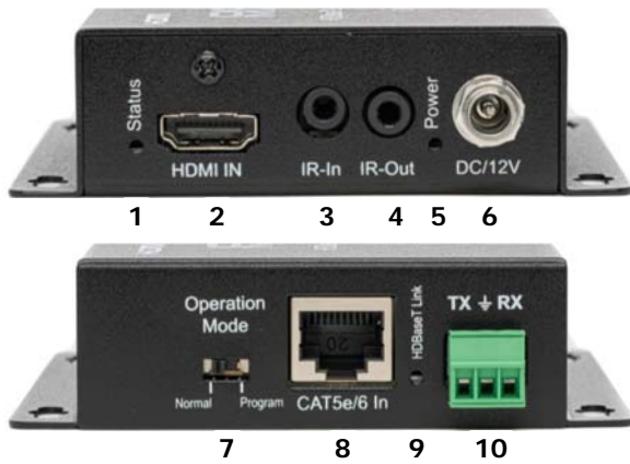
Transmitter
