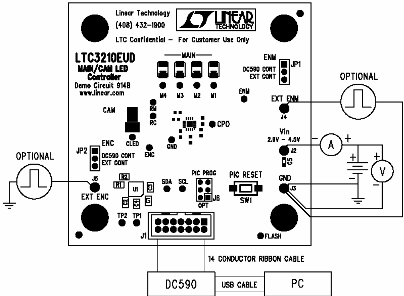
Figure 1. Proper Measurement Equipment Setup for DC914
