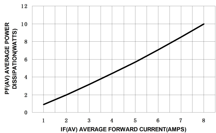
Fig.5- Power Dissipation
