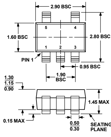
Figure 33. 5-Lead Small Outline Transistor Package [SOT-23] (RJ-5) Dimensions shown in millimeters
