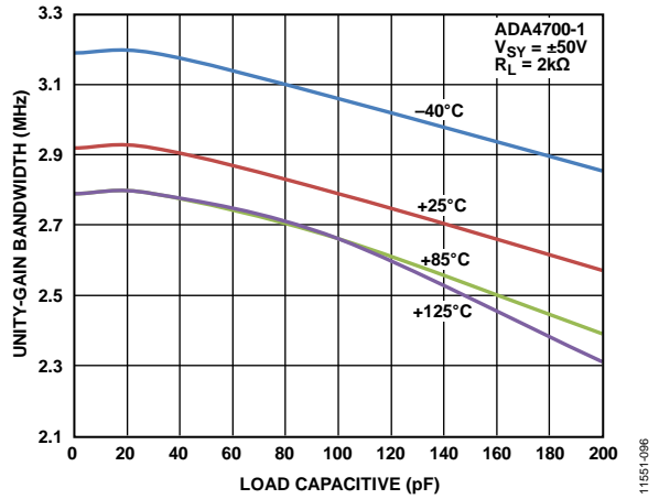
Figure 24. Unity-Gain Bandwidth vs. Load Capacitance and Temperature, V SY = ±50 V
