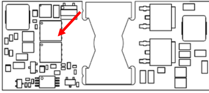
Figure 15. Temperature Monitoring Locations
