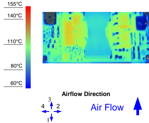
Figure 8. Thermal Image for Airflow Direction 3 (3A output, 55°C ambient, 200 LFM, typical V_{in} , open frame, unit soldered onto a fixture board)
