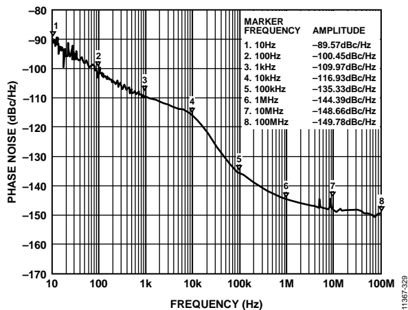
Figure 29. Additive Phase Noise with Clock Input = 1200 MHz and HSTL Outputs = 1200 MHz
