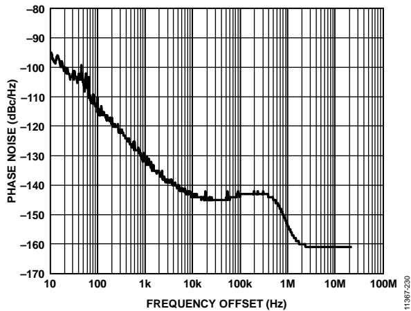
Figure 28. Absolute Phase Noise of Clock Source at 622.08 MHz
