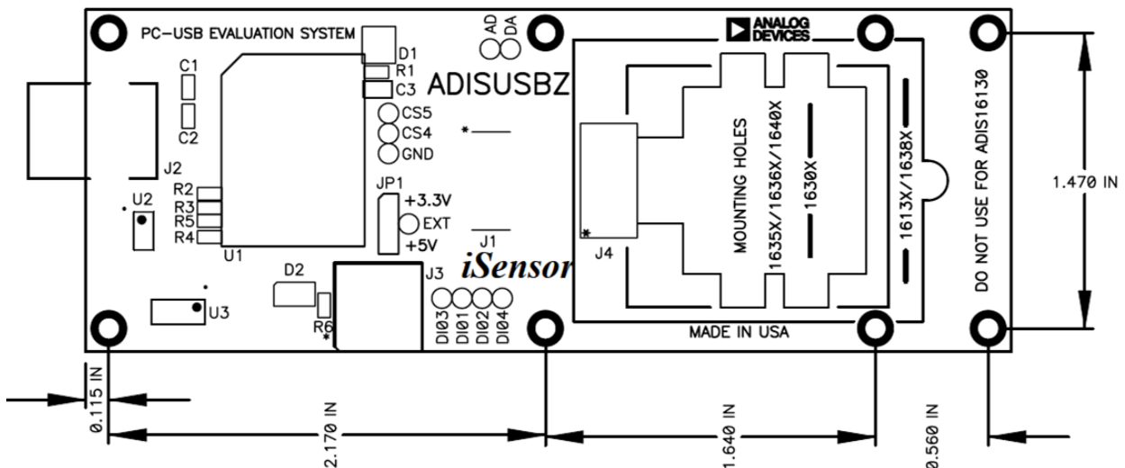
Figure 2. ADISUSBZ Top View, Dimensions and Mounting Hole Locations
