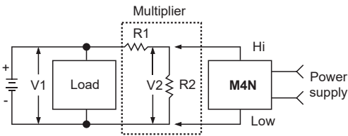
(Fig. 2) Measuring input (V1) is under 200VDC
