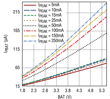
Input Quiescent Current Into PBAT Due to Gate Charge, V_{OUT} = 3.3V , Running Continuous
