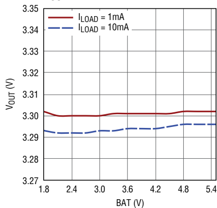
Buck-Boost Line Regulation, V_{OUT} = 3.3V , 100mA I_{PEAK} Setting
