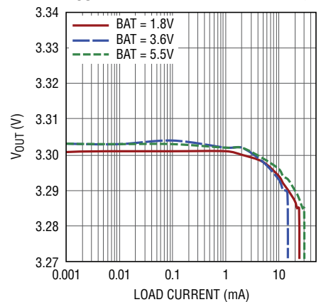
Buck-Boost Load Regulation, V_{OUT} = 3.3V , 100mA I_{PEAK} Setting
