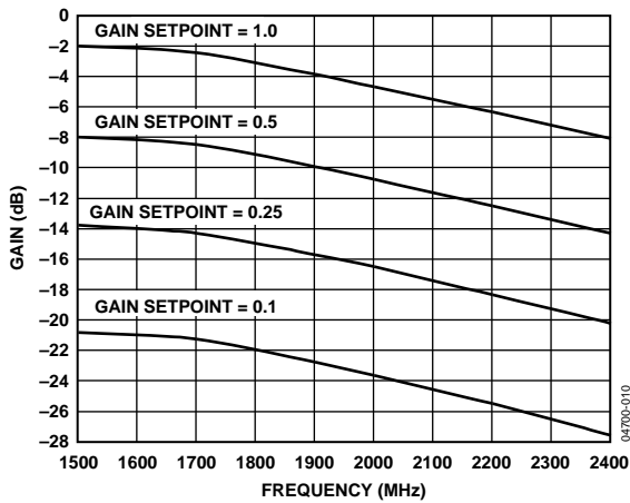
Figure 10. Gain vs. Frequency at Different Gain Setpoints, Phase Setpoint = 0^\circ
